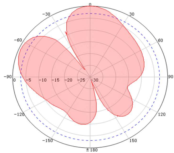
2100MHz Vertical
